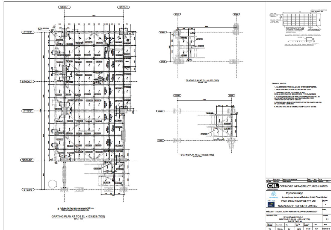
GRATING PLAN
