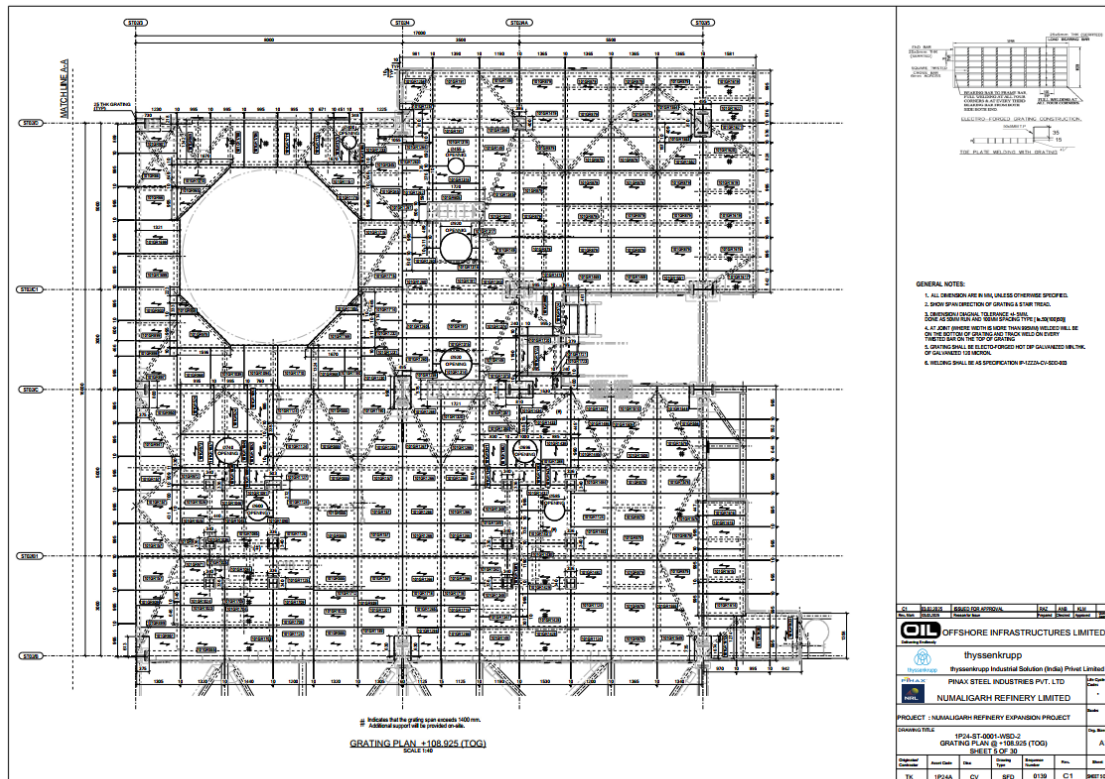
GRATING PLAN
